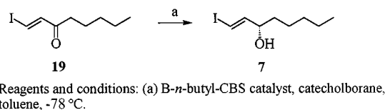
Scheme 3. Catalytic asymmetric CBS reduction of the β-iodovinyl ketone 19
